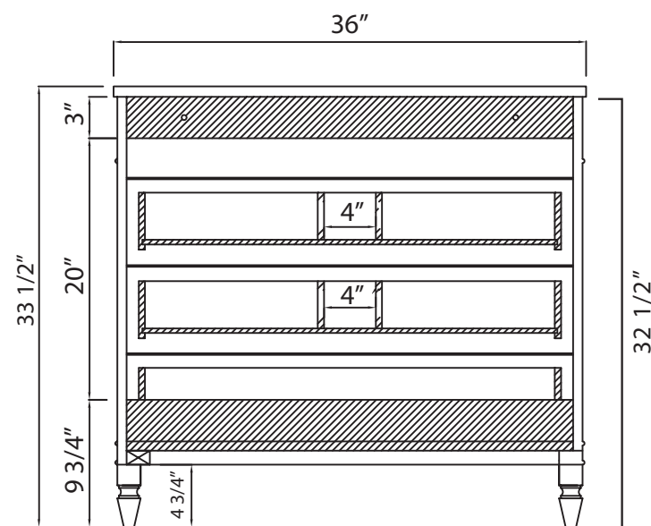
BACK VIEW
