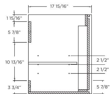
WALL HUNG
