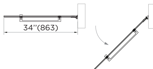
HANDLE DIMENSIONS
