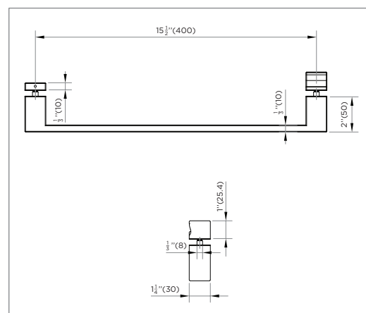
HANDLE DIMENSIONS
