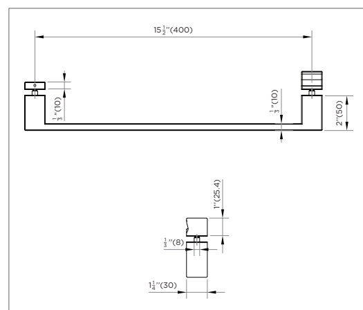
HANDLE DIMENSIONS
