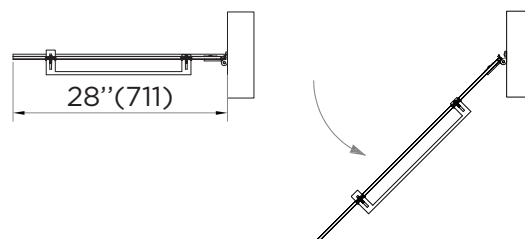
HANDLE DIMENSIONS
