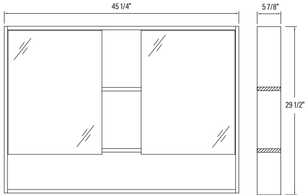
# SHMC48 45 1/4" x 5 7/8" x 29 1/2"
