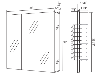
# AMA3636 36" x 36" x 5 3/8"
