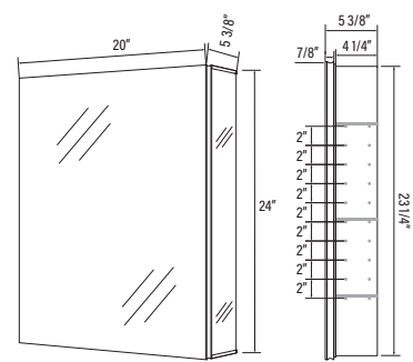
# AMA2024 20" x 24" x 5 3/8"
