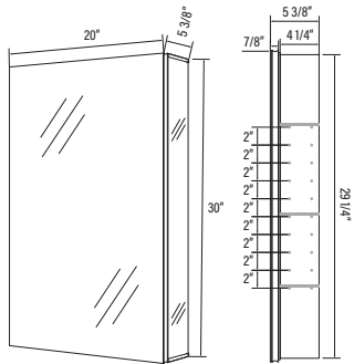
# AMA2030 20" x 30" x 5 3/8"
