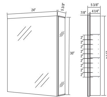
# AMA2430 24" x 30" x 5 3/8"
