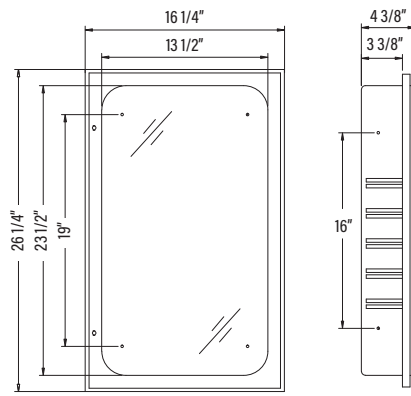
# MCB1626 16 1/4" x 26 1/4" x 4 3/8"
