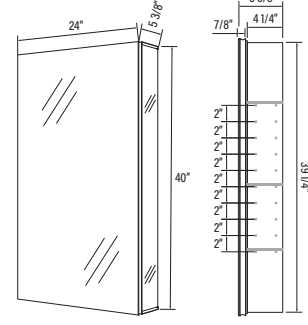
# AMA2440 24" x 40" x 5 3/8"
