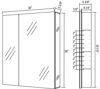
# AMA3036 30" x 36" x 5 3/8"
