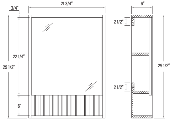
# VVMC22 21 3/4" x 29 1/2" x 5 7/8"
