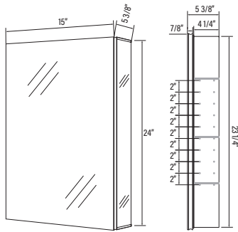
# AMA1524 15" x 24" x 5 3/8"
