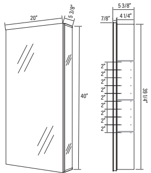
# AMA2040 20" x 40" x 5 3/8"
