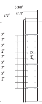
# AMB3630 36" x 30" x 5 3/8"
