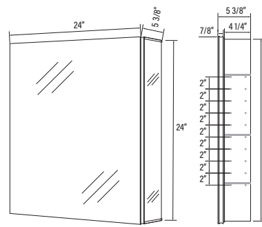
# AMA2424 24" x 24" x 5 3/8"
