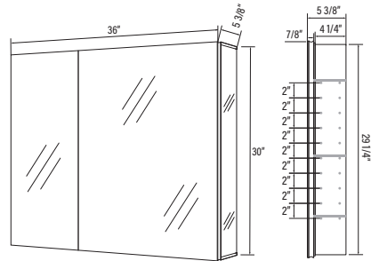
# AMA3630 36" x 30" x 5 3/8"
