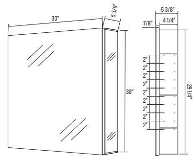
# AMA3030 30" x 30" x 5 3/8"
