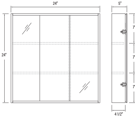
# SM2424-3 24" x 24" x 5"
