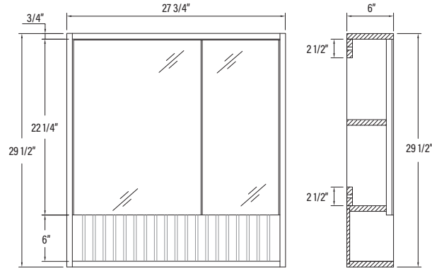
# VVMC28 27 3/4" x 29 1/2" x 5 7/8"
