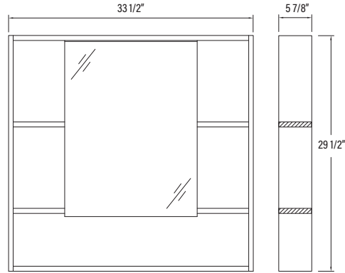
# SHMC36 33 1/2" x 5 7/8" x 29 1/2"
